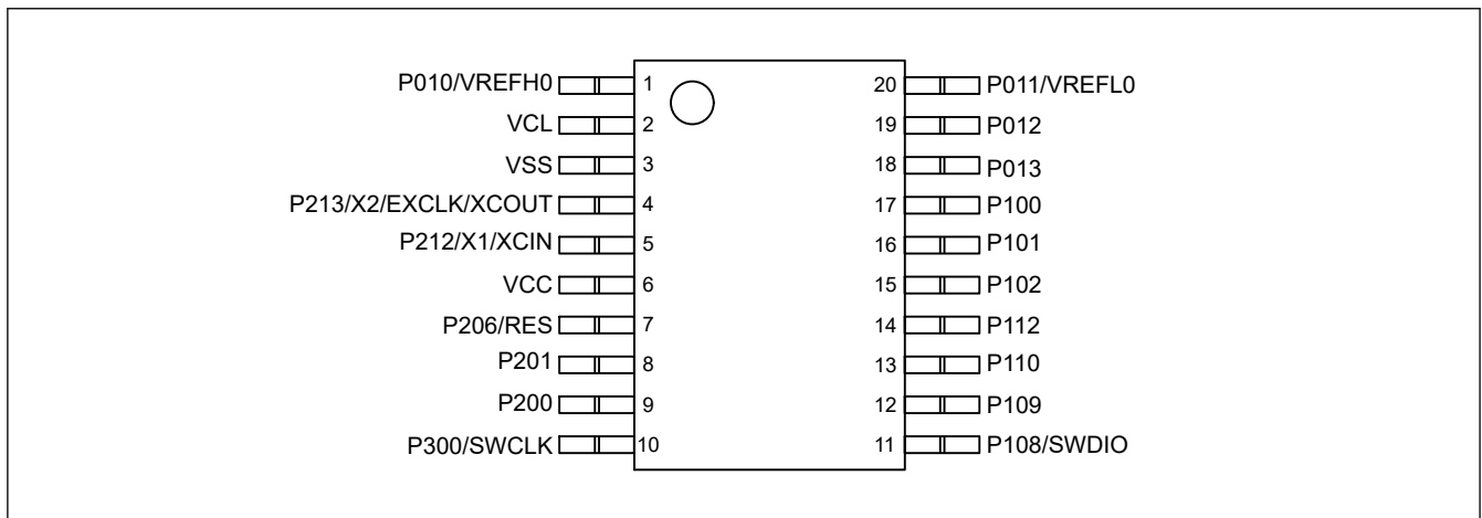
Figure 1.5 Pin assignment for LSSOP/TSSOP 20-pin (top view)
