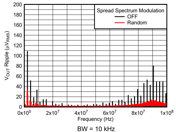
Figure 6-16. V_{OUT} Ripple FFT After the Second L-C Filter
