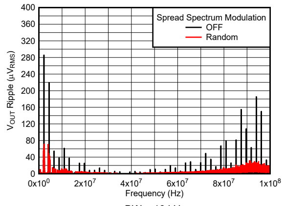
BW = 10 kHz 12 V to 3.3 V, 1 A 2.2 \mu\text{H} , 2.2 MHz First L-C Only Figure 6-10. V_{OUT} Ripple FFT After the First L-C Filter
