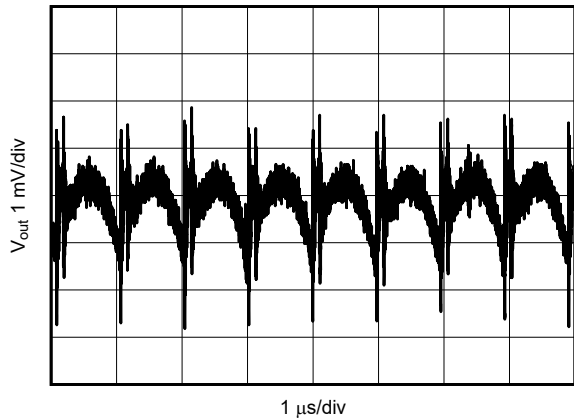
Figure 6-1. V_{OUT} Ripple After the First L-C Filter
