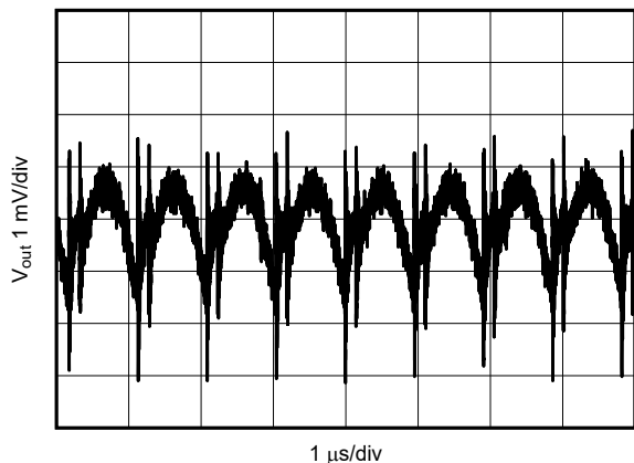
Figure 6-5. V_{OUT} Ripple After the First L-C Filter
