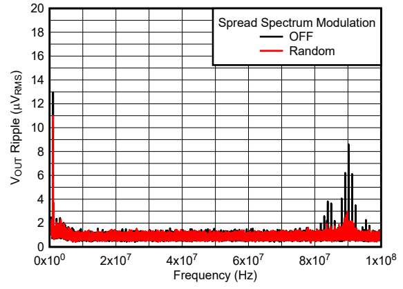
BW = 10 kHz 12 V to 1.8 V, 1 A 2.2 \mu\text{H} , 1 MHz First and second L-C Figure 6-8. V_{OUT} Ripple FFT After the Second L-C Filter
