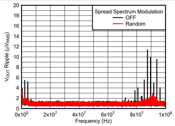
BW = 10 kHz 12 V to 3.3 V, 1 A 2.2 \mu\text{H} , 2.2 MHz First and second L-C Figure 6-12. V_{OUT} Ripple FFT After the Second L-C Filter
