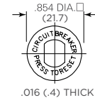
Embossed Aluminum
