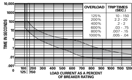
CURVE 2 STANDARD DELAY 50/60 Hz.
