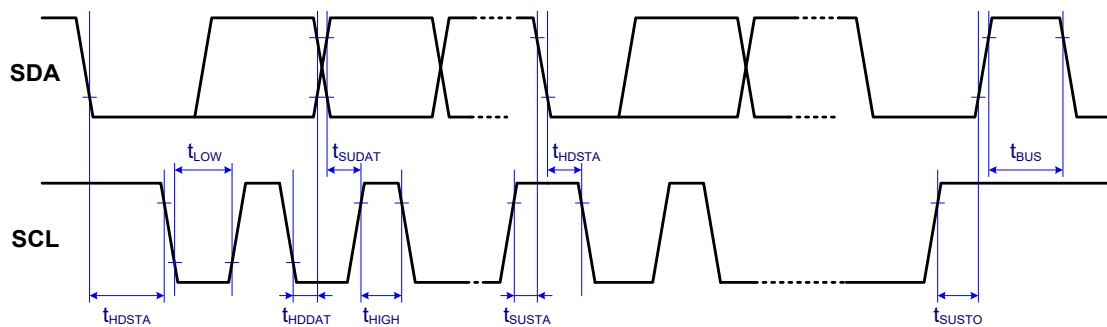
Figure 8. Bus Timing
