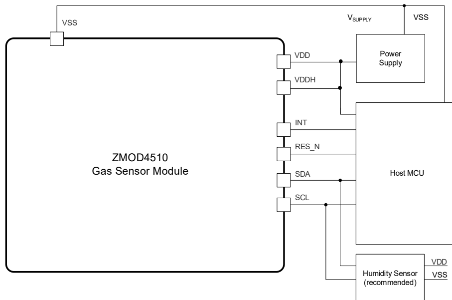
Figure 3. Application Circuit
