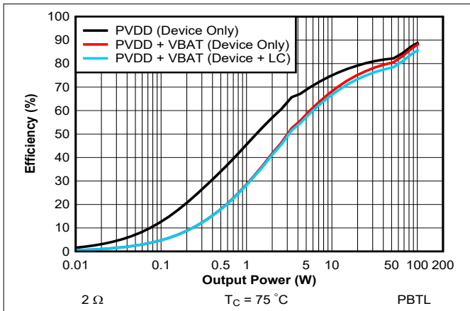
Figure 7-34. Efficiency vs Output power - PBTL - 2 \Omega (Zoomed)
