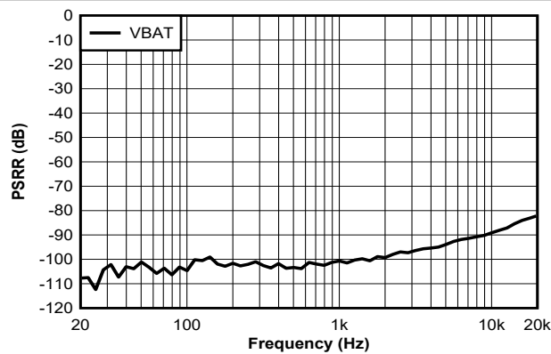
Figure 7-17. PSRR vs Frequency - VBAT Only
