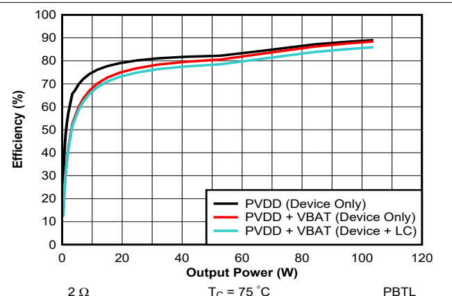
Figure 7-33. Efficiency vs Output Power - PBTL - 2 Ω
