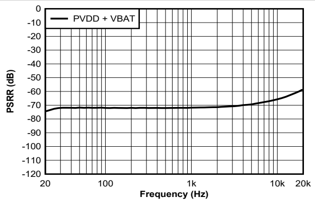
Figure 7-18. PSRR vs Frequency - PVDD + VBAT
