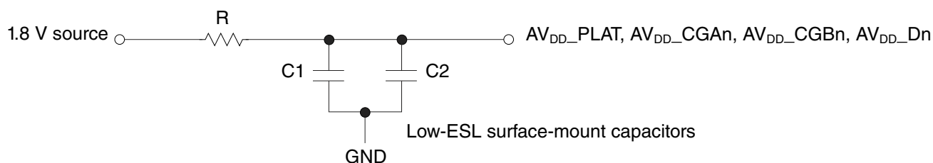
Figure 53. PLL power supply filter circuit
