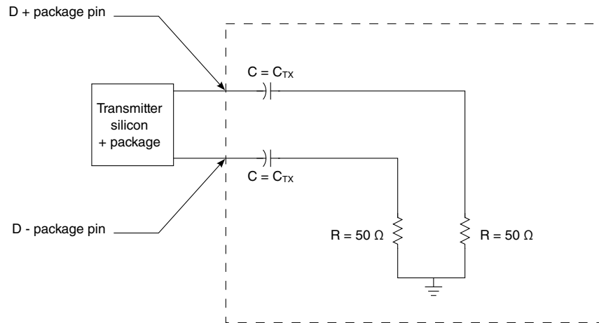
Figure 40. Test/measurement load
