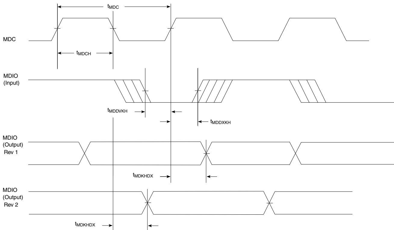
Figure 16. Ethernet management interface timing diagram
