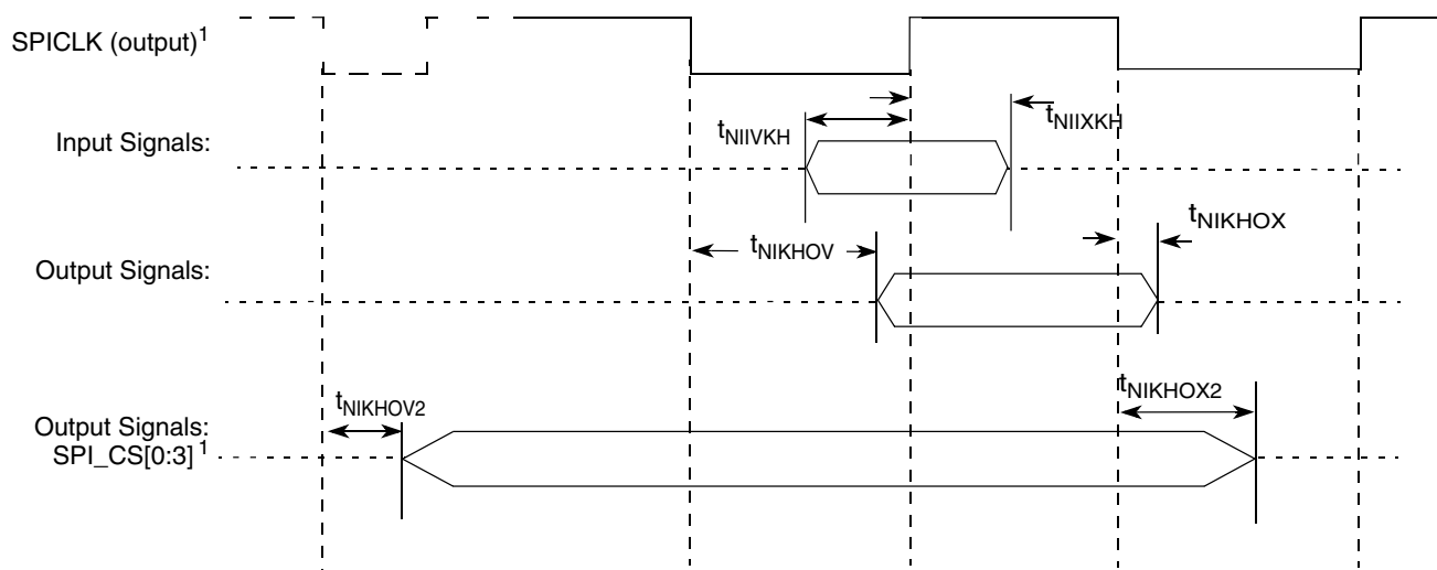
Figure 14. eSPI AC timing in master mode (internal clock) diagram
