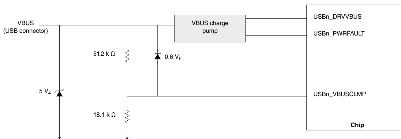
Figure 65. Divider network at VBUS
