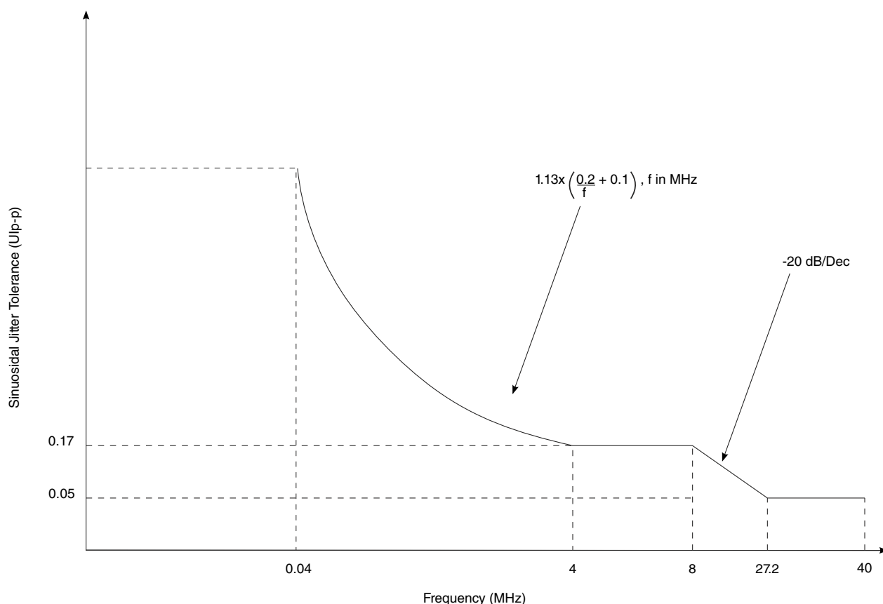
Figure 48. XFI host receiver input sinusoidal jitter tolerance
