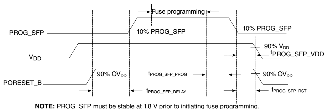
Figure 8. PROG_SFP timing diagram
