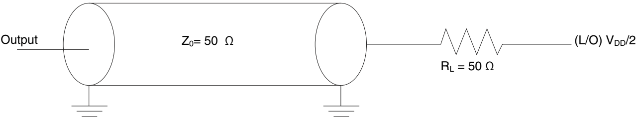
Figure 30. GPIO AC test load
