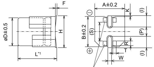
*1 : E to G : L±0.3 Supportive Terminals ( ) Reference size
