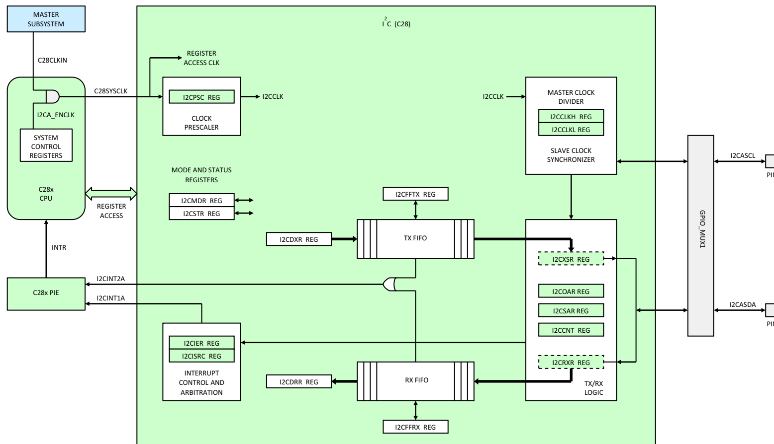
Figure 5-49. I2C (C28x)
