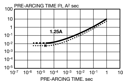
Fig. 4c. Choice of 1.25A fuse, example #4.
