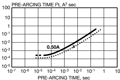
Fig. 3c. Choice of 0.5A fuse, example #3.
