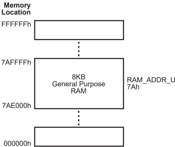
Figure 46.eZ80F92 On-Chip RAM Memory Addressing Example
