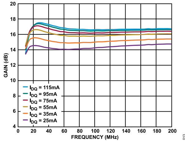
Figure 13. Gain vs. Frequency for Various I_{DQ} Values, 10 MHz to 200 MHz, V_{DD} = 5\text{ V}
