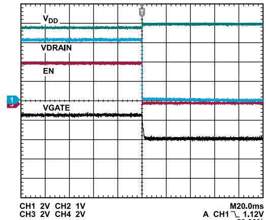
Figure 58. Turn Off HMC980LP4E Outputs to ADPA7005CHIP
