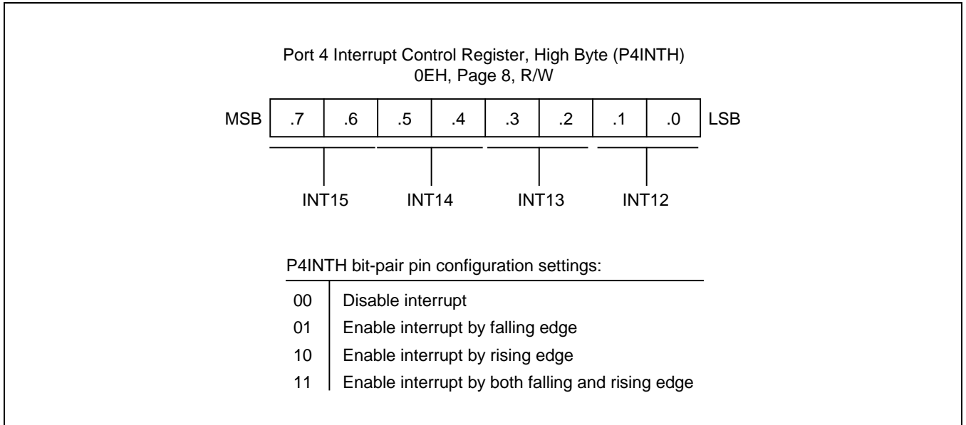
Figure 9-20 Port 4 High-Byte Interrupt Control Register (P4INTH)
