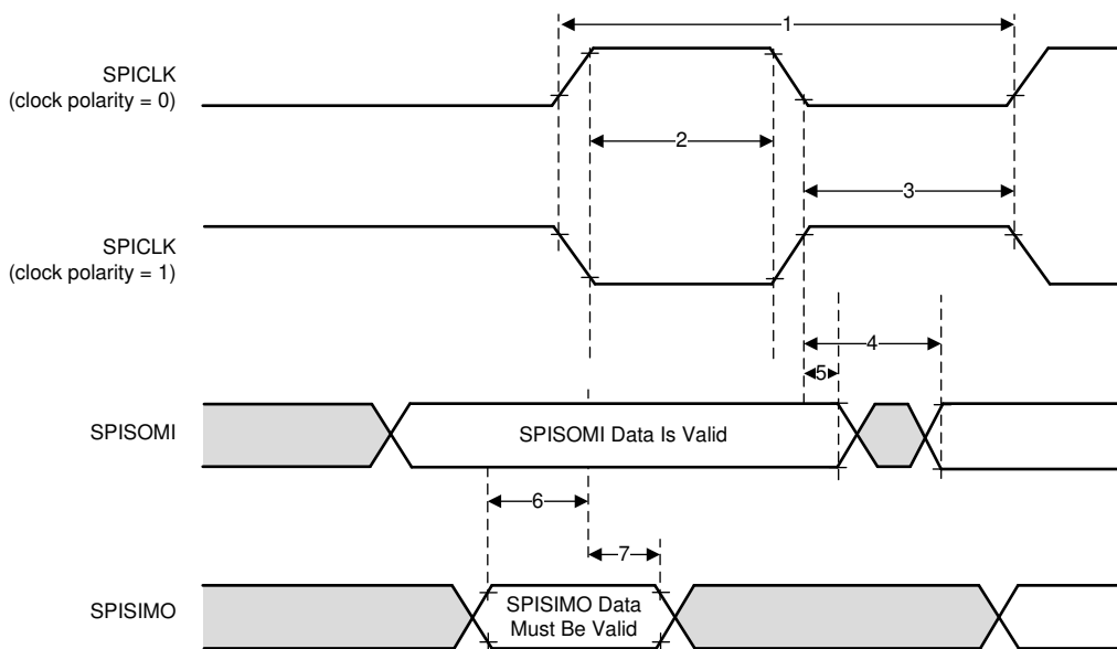
Figure 7-10. SPI peripheral Mode External Timing (CLOCK PHASE = 1)
