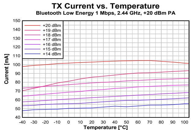
Figure 7-13. TX Current vs. Temperature (Bluetooth Low Energy 1 Mbps, 2.44 GHz, VDD5 = 3.3 V)
