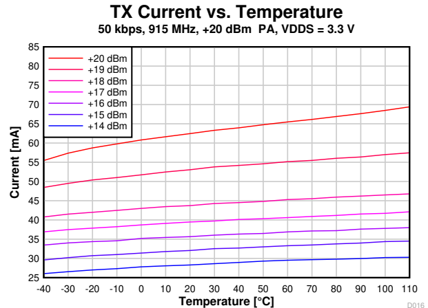
Figure 7-11. TX Current vs. Temperature (50 kbps, 915 MHz, VDD5 = 3.3 V)
