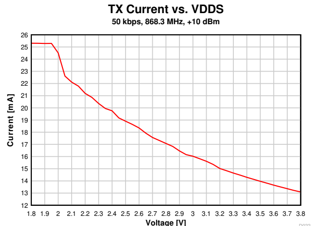
Figure 7-15. TX Current vs. Supply Voltage (VDD5) (50 kbps, 868.3 MHz)
