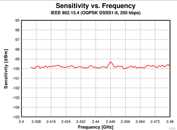
Figure 7-23. Sensitivity vs. Frequency (250 kbps, 2.44 GHz)
