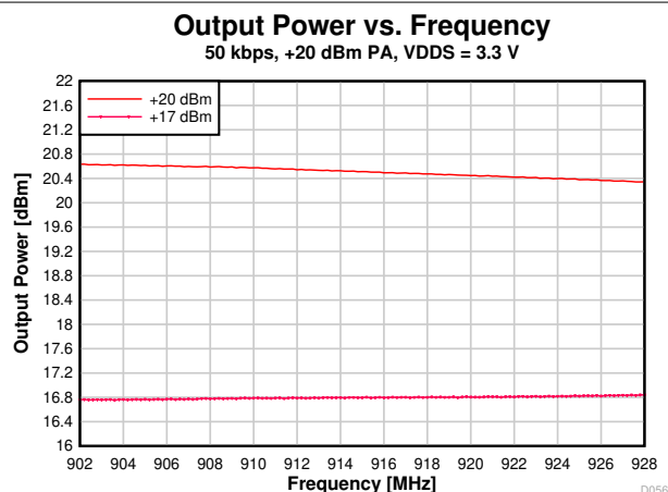
Figure 7-49. Output Power vs. Frequency (50 kbps, 915 MHz, VDD5 = 3.3 V)
