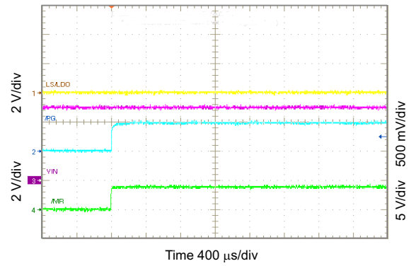
Figure 10-62. \overline{\text{PG}} Functions as Shifted \overline{\text{MR}} Output
