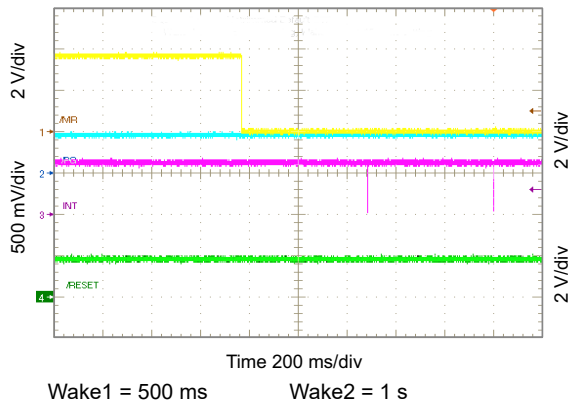
Figure 10-63. Show \overline{\text{MR}} Timing
