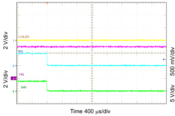
Figure 10-61. \overline{\text{PG}} Functions as Shifted \overline{\text{MR}} Output
