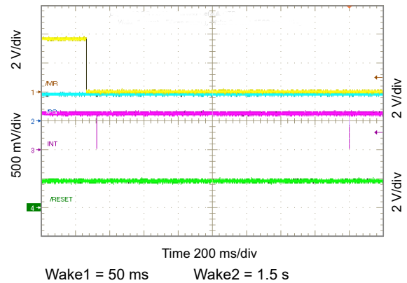
Figure 10-64. Show \overline{\text{MR}} Timing
