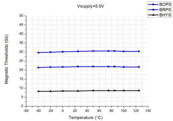
Magnetic threshold value vs temperature @ VDD=5.5\text{v}
