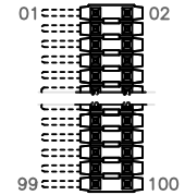
DOUBLE ROW TOP VIEW
