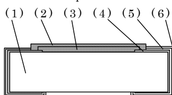
a-a' sectional plan
