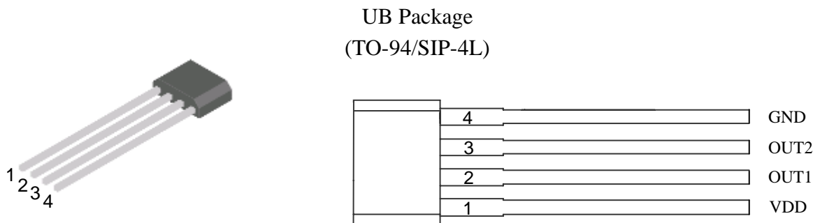
Figure 2. Pin Configuration of GH686A (Front View)
