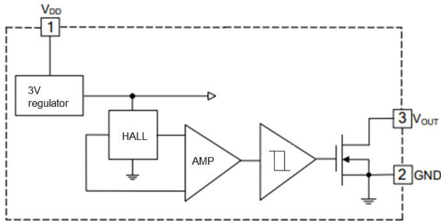
Figure 2. Block Diagram
