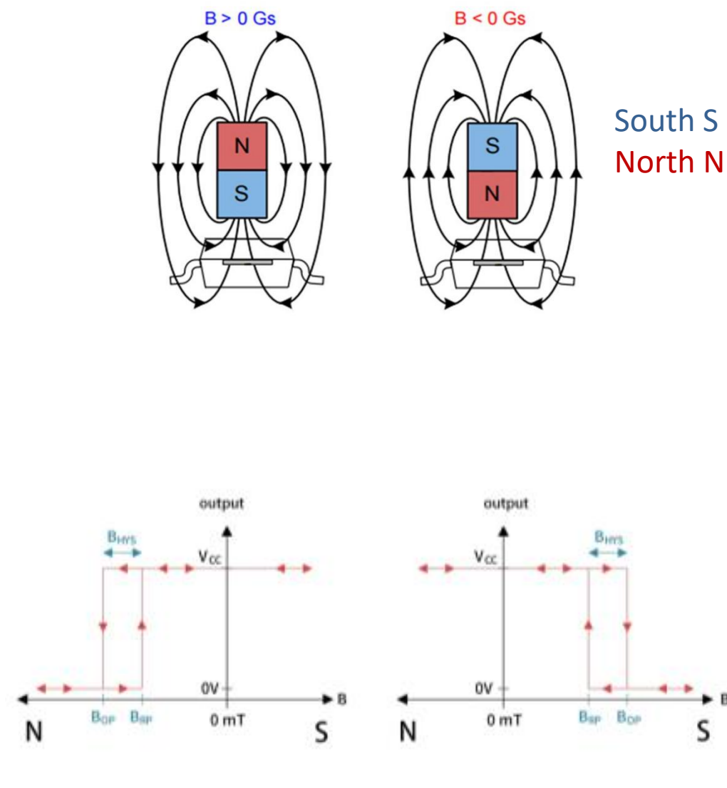
Figure 3. Output characteristics
