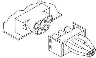
System 5 Cable to Right Angle (90°) Board Mount
