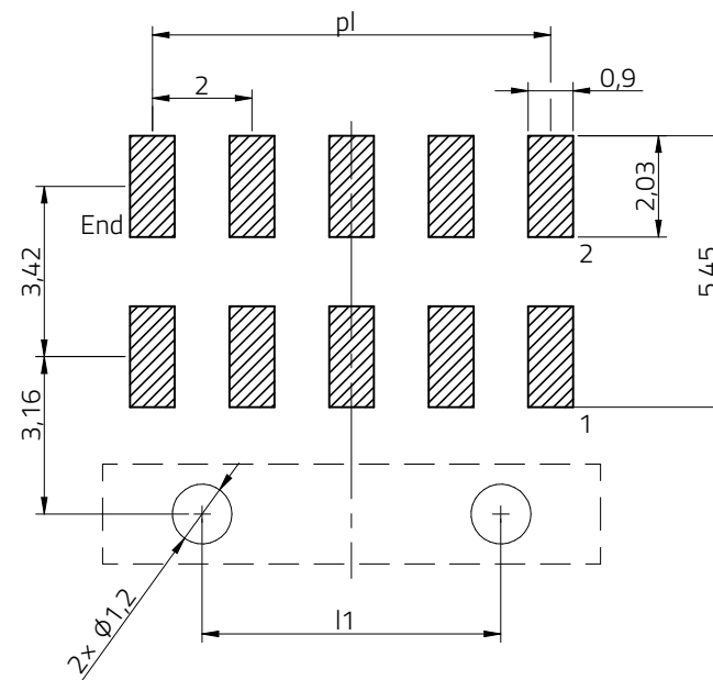
Recommended PCB Layout General tolerance \pm 0.05
