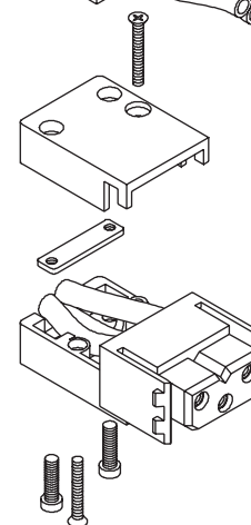
System 9 Cable Connector with Cable Adapter
