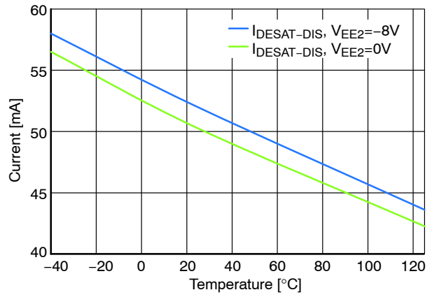
Figure 29. Desat Discharge Current
