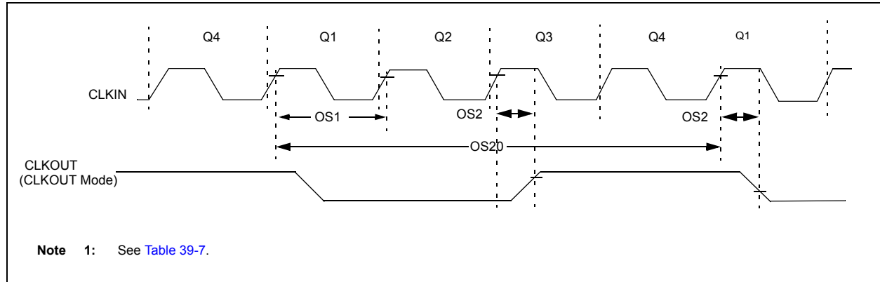
FIGURE 39-5: CLOCK TIMING
