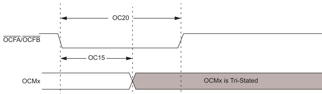
Figure 30-8. MCCP PWM Mode Timing Characteristics
