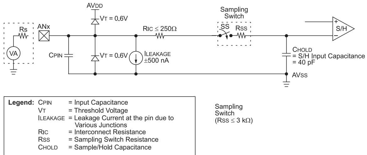
Figure 21-3. 12-Bit A/D Converter Analog Input Model
