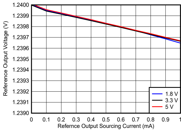
Figure 6-17. Reference Voltage vs. Reference Output Sourcing Current
