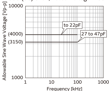
Chip (L×W): 4.5×2.0mm COG (5C) Char., Rated Voltage: DC3.15kV
