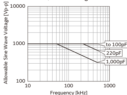
Chip (L×W): 3.2×1.6mm COG char., Rated Voltage: DC1kV
