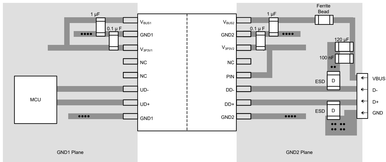
Figure 11-1. Layout Example for ISOU5B111
