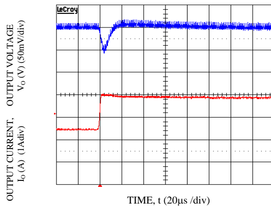
Figure 22. Transient Response to Dynamic Load Change from 50% to 100% at 12 Vin, Cout-2x47 \mu F, CTune-2700 pF & RTune-261 \Omega . Vo = 2.5 V
