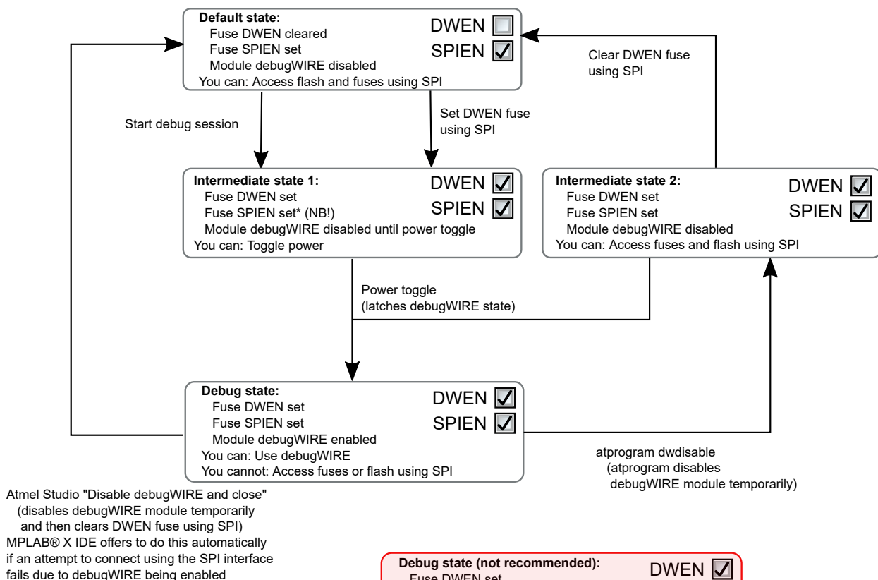
Figure 4-1. Understanding debugWIRE and the DWEN Fuse
