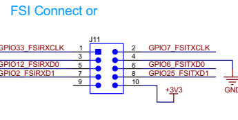
Figure 5. MCU025B_Connectors.SchDoc
