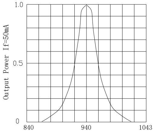
Fig.1 Relative Luminous Intensity VS. Wavelength (nm)
