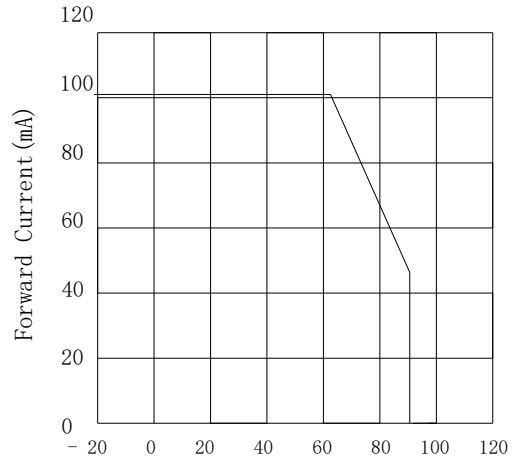
Fig.2 Forward Current VS. Ambient Temperature (°C)
