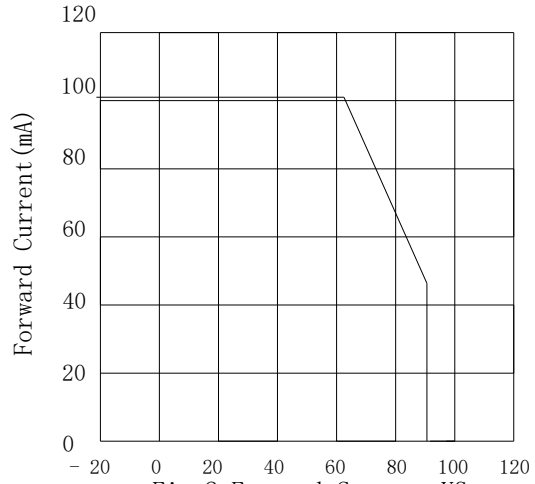
Fig. 2 Forward Current VS. Ambient Temperature (°C)
