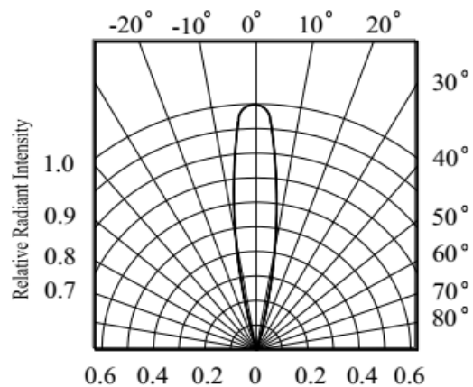
Relative Radiant Intensity vs. Angular Displacement
