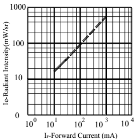
Radiant Intensity vs. Forward Current
