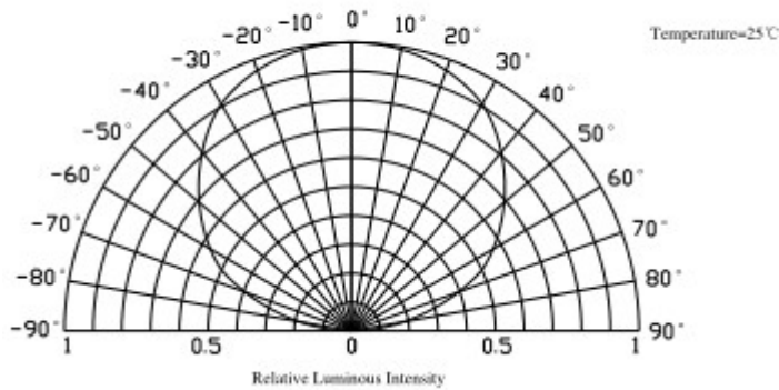
Radiation Diagram
