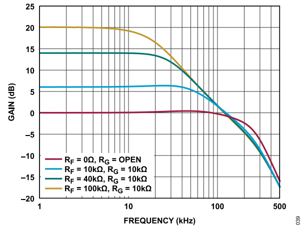
Figure 41. Noninverting Small Signal Frequency Response
