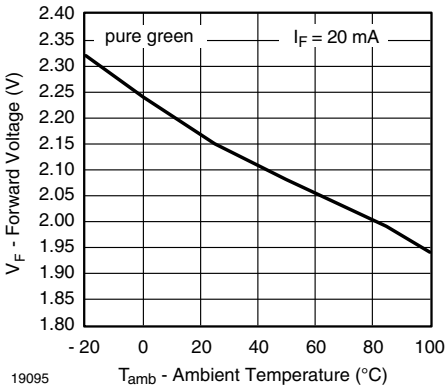
Fig. 32 - Forward Voltage vs. Ambient Temperature
