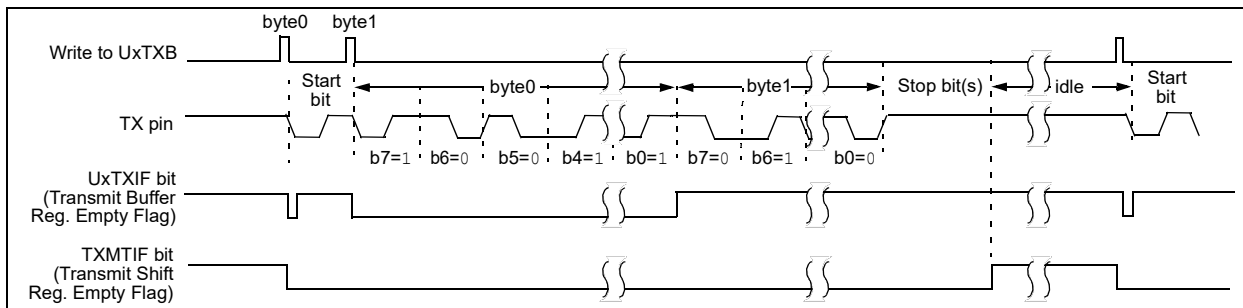
FIGURE 31-7: MANCHESTER TIMING
