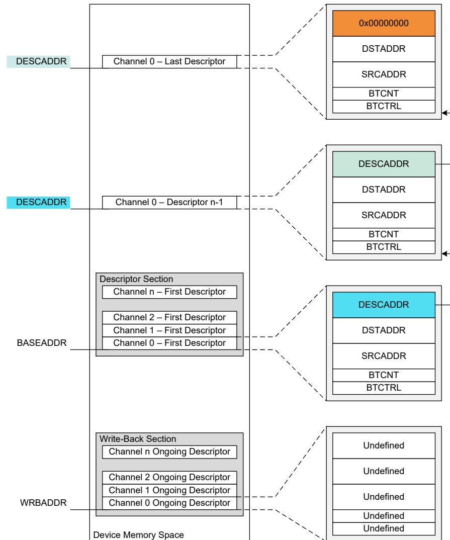
Figure 22-3. Memory Sections
