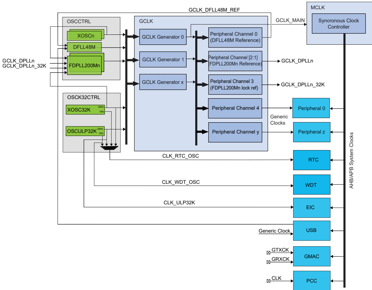
Figure 13-1. Clock Distribution
