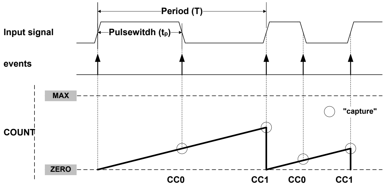
Figure 48-13. PWP Capture
