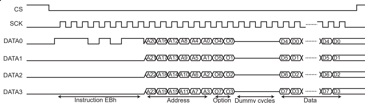
Figure 37-9. Instruction Frame
