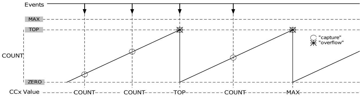
Figure 48-15. Time Stamp
