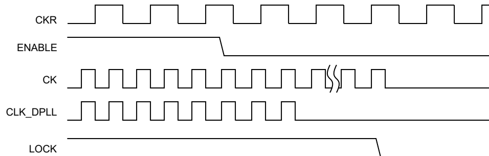
Figure 28-6. CK and CLK_DPLL Output from Running Mode to DPLLC Off Mode.
