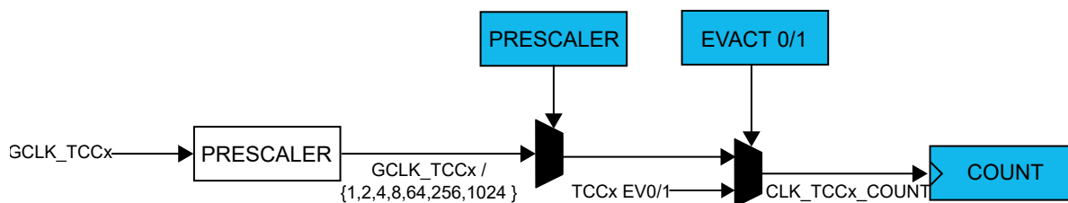
Figure 49-2. Prescaler
