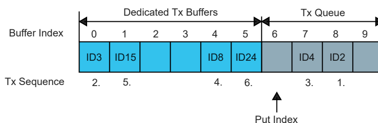
Figure 39-11. Example of mixed Configuration Dedicated Tx Buffers / Tx Queue
