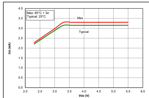
FIGURE 38-6: I_{DD} , HFINTOSC Mode, FOSC = 32 MHz, PIC16F15324/44 Only.
