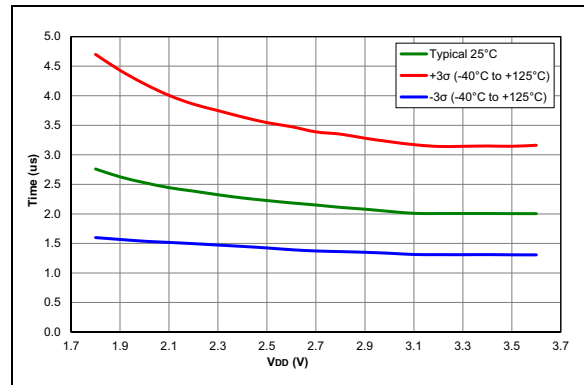
FIGURE 38-66: ADC RC Oscillator Period, PIC16LF15324/44 Only.
