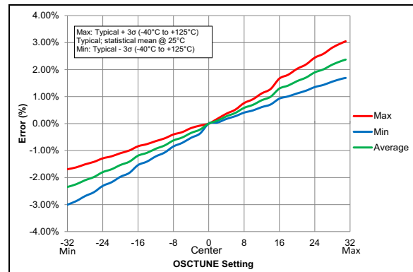
FIGURE 38-105: OSCTUNE Center Frequency, PIC16LF15324/44 Only.
