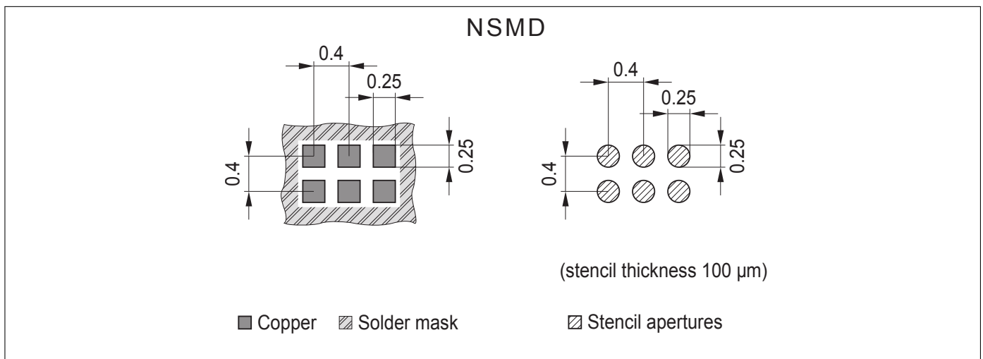
Figure 5: Footprint recommendation
