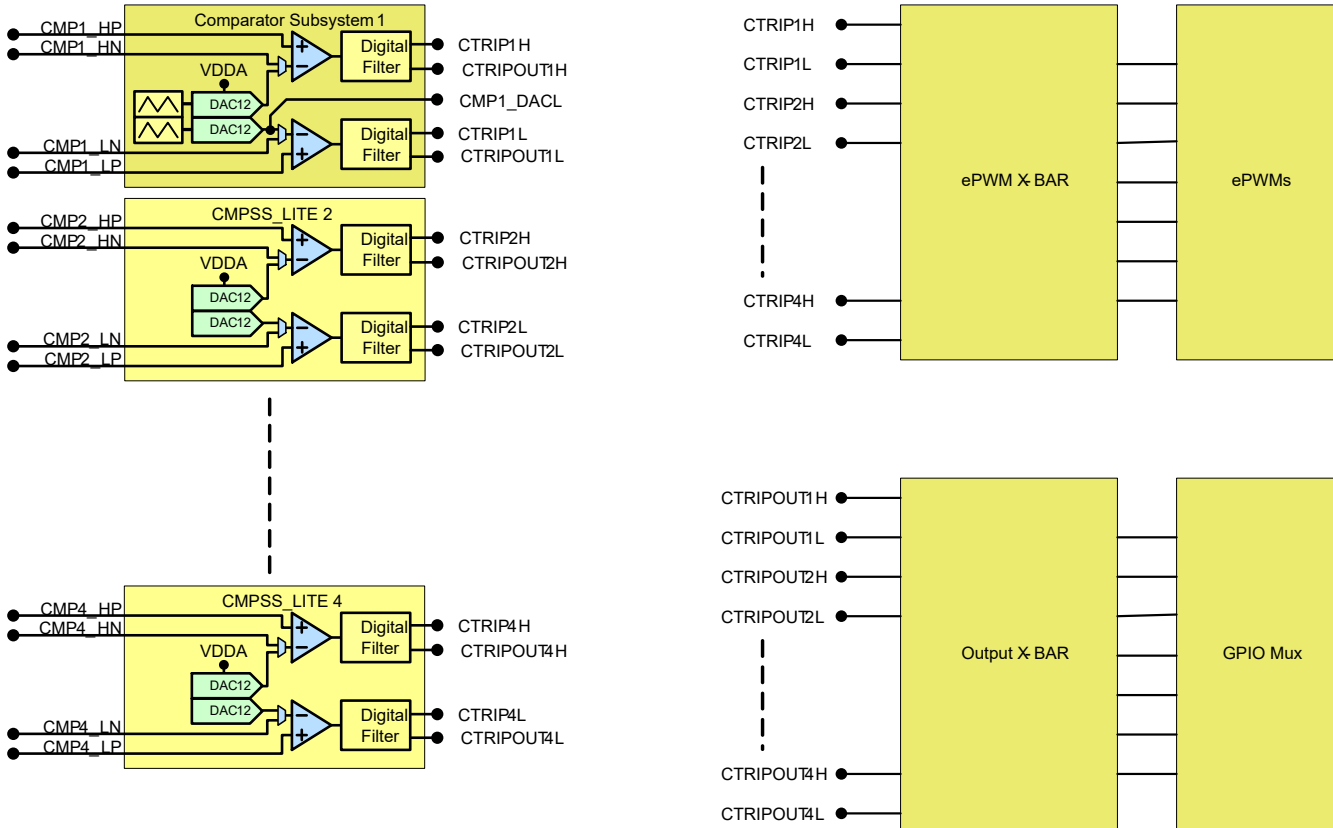
Figure 6-45. CMPSS Connectivity
