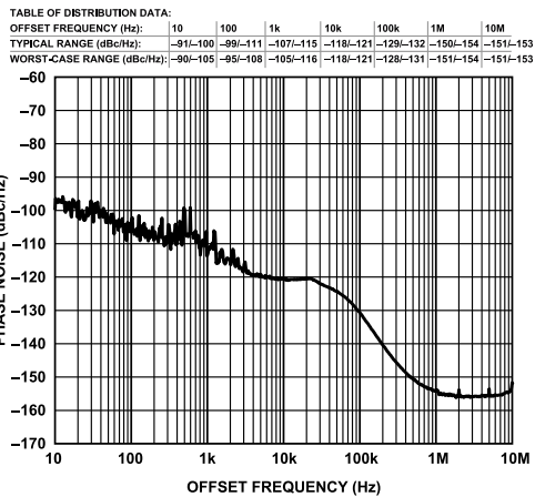
Figure 37. Phase Noise Performance Including Distribution Table at LO Frequency = 100 MHz at Nominal and Worst-Case Conditions
