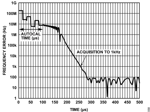
Figure 58. PLL Acquisition
