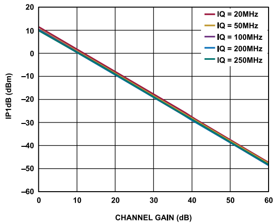
Figure 12. Input 1dB Compression Point (IP1dB) vs. Channel Gain, and IQ Output Frequency, LO = 1000 MHz, Nominal Conditions, Wideband Mode
