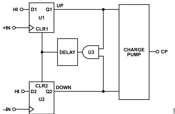
Figure 56. PFD Simplified Schematic
