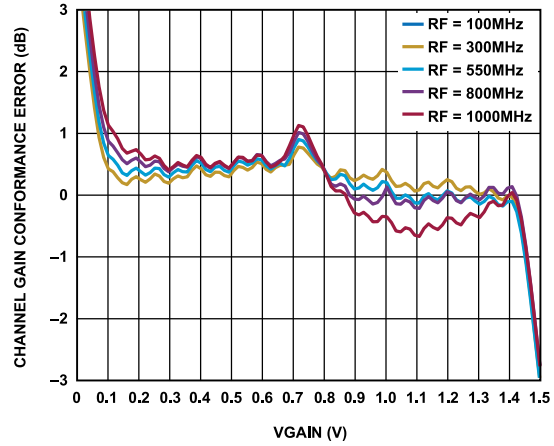
Figure 32. Channel Gain Conformance Error vs. V_{GAIN} and RF Input Frequency, Nominal Conditions
