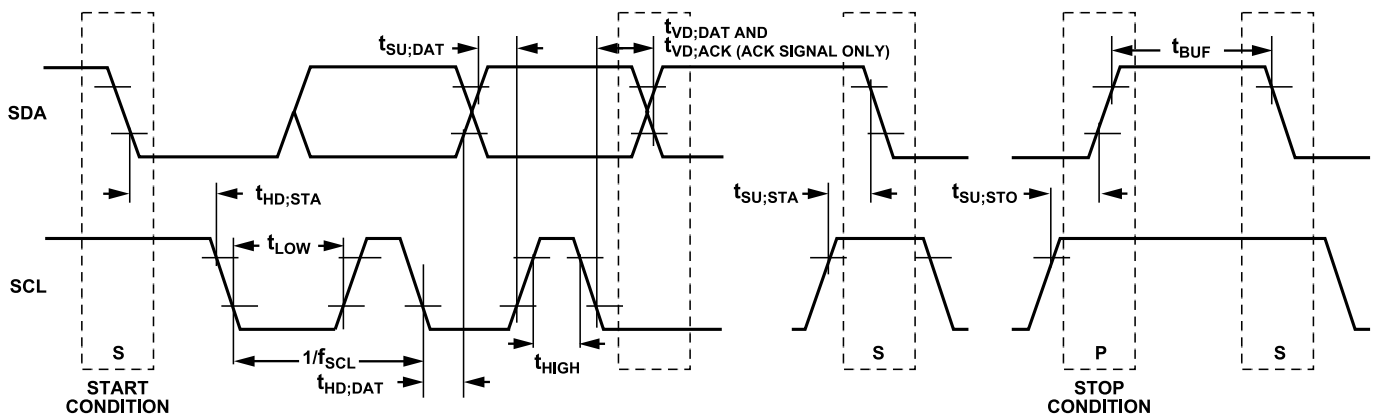
Figure 2. I 2 C Port Timing Diagram
