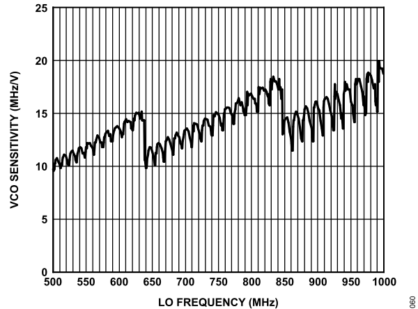
Figure 60. K_{VCO} vs. LO Frequency
