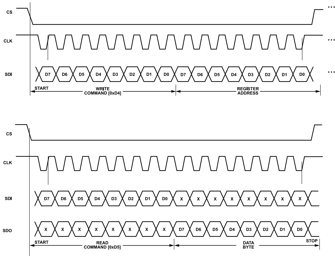
Figure 67. SPI Byte Read Example
