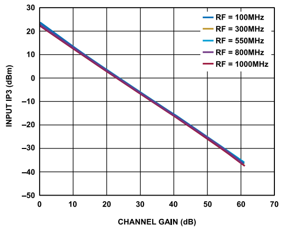
Figure 13. Input IP3 vs. Channel Gain, and RF Input Frequency, Nominal Conditions
