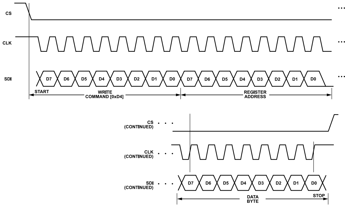
Figure 66. SPI Byte Write Example
