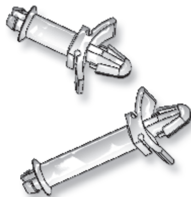
"LSP" SERIES - MSP END FITS A .156" HOLE LOCKING END FITS .187" HOLE PANEL THICKNESS .030 / .078
