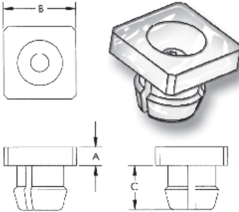
PART NUMBER 401003
