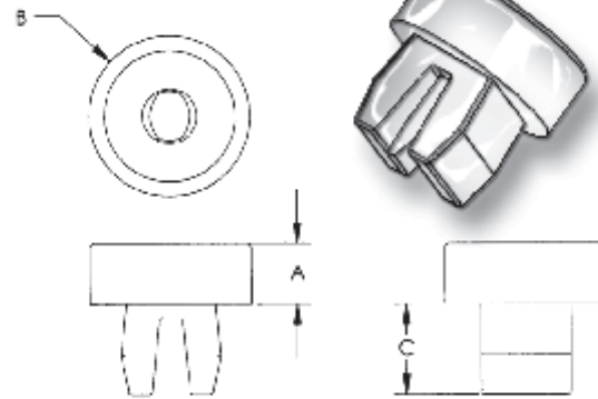
PART NUMBER 401021
