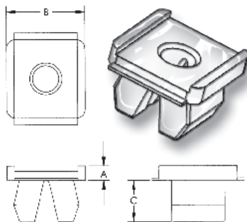
PART NUMBER 401025
