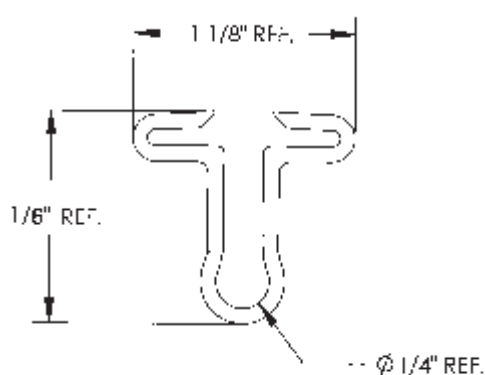
CLOSED LOOP
