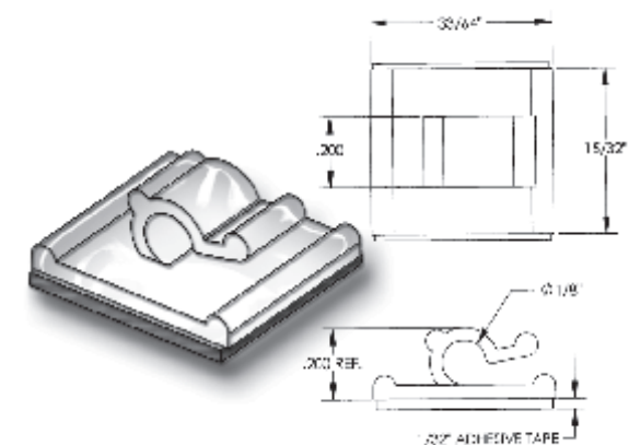
PART NUMBER 22AWC00125
