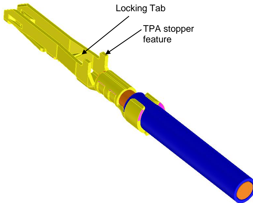
Single Row Receptacle – Terminal position into the housing
