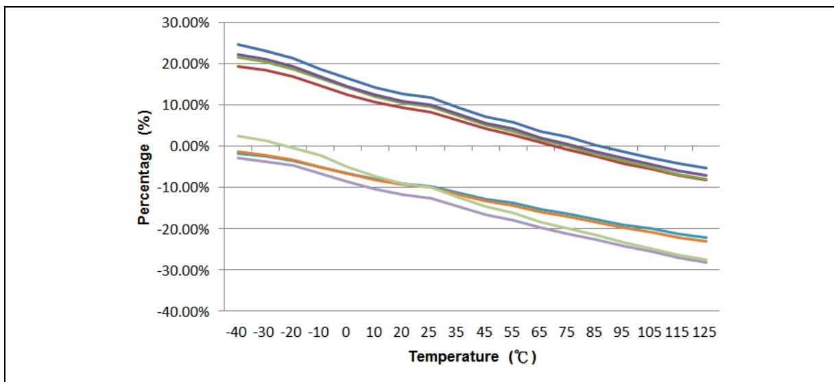
Figure 7.3-3 LIRC deviation under V_{DD} = 5.5\text{ V}
